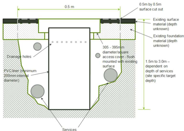
Figure 2. Schematic arrangement of a Ground Access Portal (GAP)
